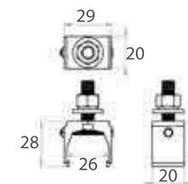
W-Type Anchor Clamp Material – GFN 30%
